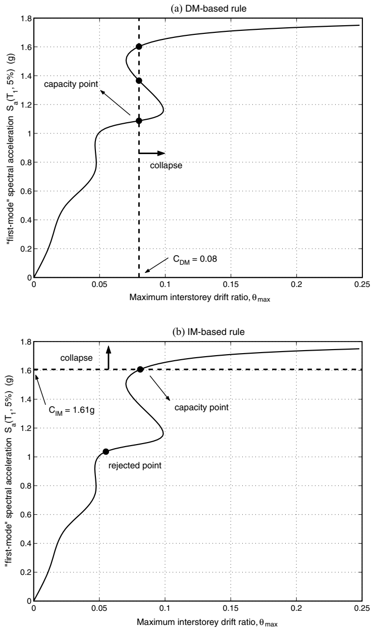
Figure 6. Two different rules producing multiple capacity points for a T_1=1.3 s, 3-storey steel moment-resisting frame with fracturing connections. The DM rule, where the DM is \theta_{max} , is set at C_{DM}=0.08 and the IM rule uses the 20% slope criterion.
